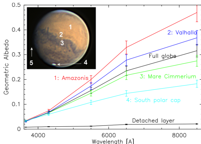
Fig. 12. Albedo of different Martian structures compared to those of the full globe and of the observed terminator feature for 17 November using a 305 mm F/5 Newtonian and an ASI183 mm Pro Camera (credit CP). From top to bottom: Amazonis (red line), Valhalla (dark blue line), full globe (black line), Mare Cimmerium (green line), south polar cap (light blue line), and the studied detached layer (black line). These values are corrected from orbital parameters: solar phase angle of 27^\circ , rotation angle 192^\circ , orbital longitude ( L_s ) 316^\circ . From left to right, the UV filter covers the range [3250–4000 Å], the blue filter [3780–4750 Å], the green filter [4780–6025 Å], the red filter [5870–7120 Å], and the IR filter [7250–10 000 Å]. Their normalised magnitudes for \alpha = 0^\circ are 0.87 (UV), -0.04 (B), -1.61 (G), -2.45 (R), and -3.09 (IR).
